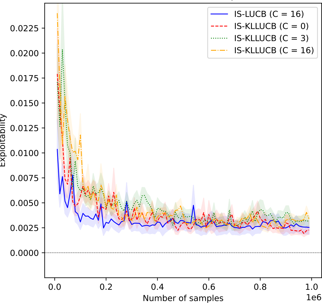
Leduc Poker, KLUCB, Player x
